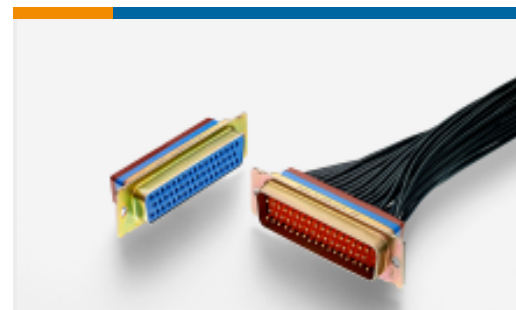
TE Part # 1-2157480-4 AMPLIMITE IP67, SZ4, 109, 37 POS, IFS, PLUG
