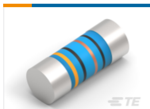
TE Part #1-2176314-8 MELF SMA_A 2K7 0.1% 15PPM 0102 0.3W
