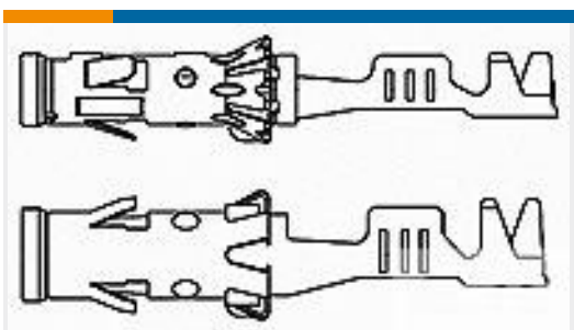
TE Part #1488991-5 3POS, MCON 1.2 CB REC 2p TL SEALED
