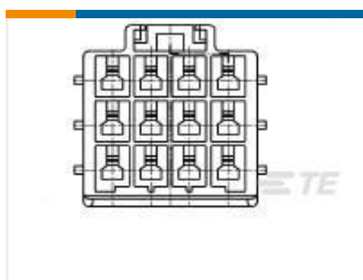
TE Part #1903720-1 PDL 3.96MM PITCH CAP HSG 12P(F)
