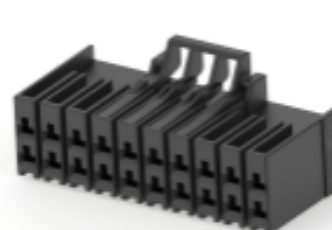
TE Part # CAT-D9934-A75C Receptacle and Tab Housing: 5.08 mm pitch, 600V
