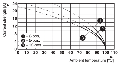
Type: FKCT 2,5/...-ST-5,08 with CCVA 2,5/...-G-5,08 P...THR
