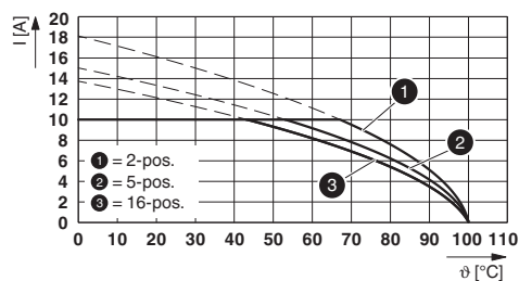
Type: FKCT 2,5/...-ST-5,08 with MDSTBVA 2,5/...-G-5,08
