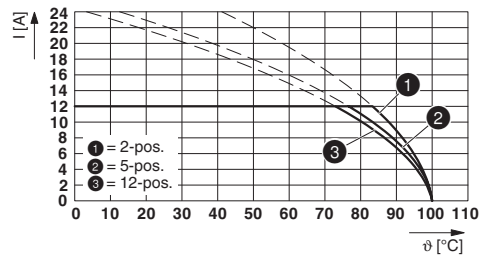
Type: FKCT 2,5/...-ST-5,08 with CC 2,5/...-G-5,08 P...THR
