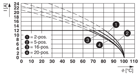
Type: FKCT 2,5/...-ST-5,08 with SMSTBA 2,5/...-G-5,08
