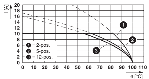
Type: FKCT 2,5/...-ST-5,08 with MDSTBW 2,5/...-G-5,08
