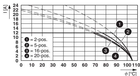
Type: FKCT 2,5/...-ST-5,08 with MSTBW 2,5/...-G-5,08
