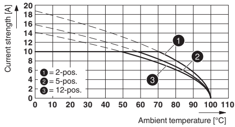
Type: FKCT 2,5/...-ST-5,08 with MDSTBV 2,5/...-G-5,08
