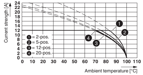
Type: FKCT 2,5/...-ST-5,08 with SMSTB 2,5/...-G-5,08
