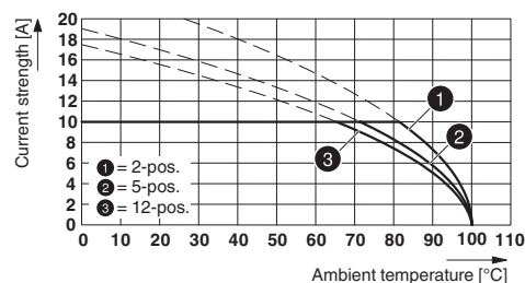
Type: FKCS 2,5/...-ST-5,08 with MDSTBV 2,5/...-G-5,08
