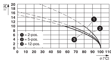
Type: FKCT 2,5/...-ST-5,08 with MDSTBA 2,5/...-G-5,08
