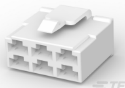
TE Part # 171898-1 FF 250 PLUG HSG 6P NYLON NAT
