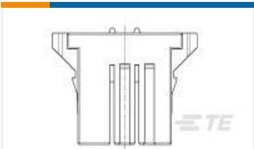
TE Part #1-1565878-3 DYNAMIC3200 SINGLE REC HSG 3P SEQUENTIAL
