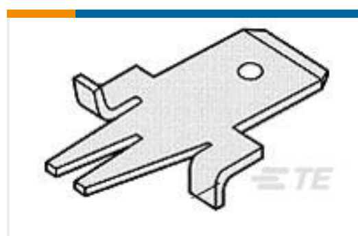
TE Part #63066-1 250 FASTON TAB TPBR
