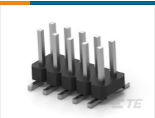
TE Part #2842142-5 10P,2MM,BRK HDR,DRVT,SMD,0.1AU, TR W/CAP
