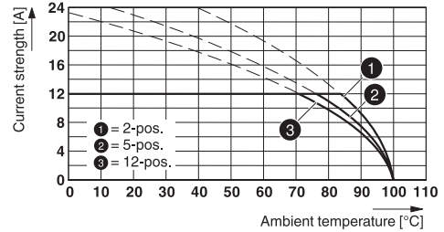
Type: FKC 2,5/...-ST-5,08 with CCA 2,5/...-G-5,08 P26THR
