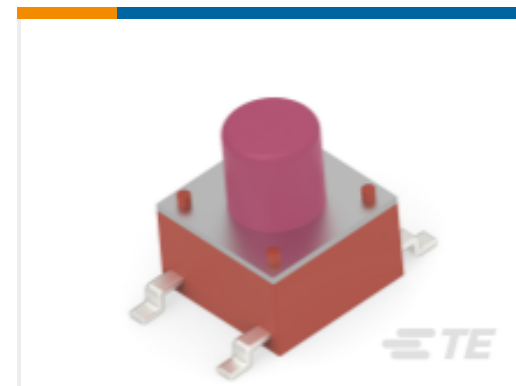
TE Part #2-1977223-0 FSM6JSMASTR=6MM TACT SWITCH, SMT 260gf,
