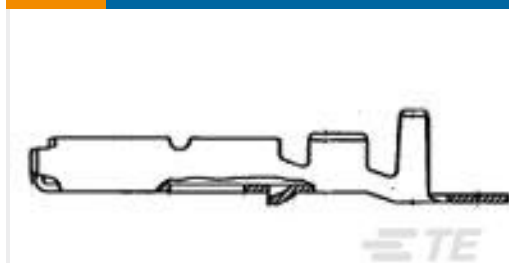
TE Part #170048-2 FASTON 110 20-24AWG TPBR
