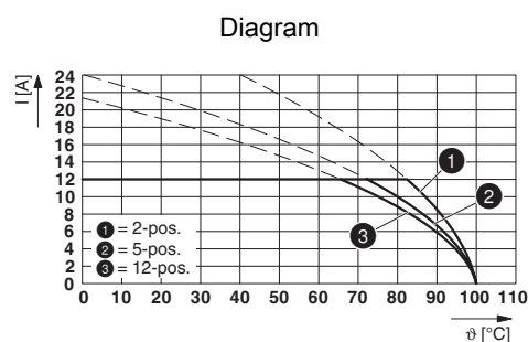
Type: MSTB 2,5/...-STF-5,08 with CCV 2,5/...-GF-5,08-LR P...THR
