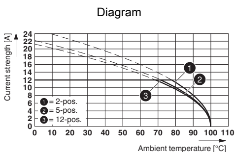
Type: MSTB 2,5/...-STF-5,08 with CCV 2,5/...-GF-5,08 P26THR
