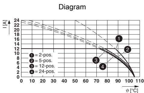
Type: MSTB 2,5/...-STF-5,08 with CC 2,5/...-GF-5,08-LR P...THR
