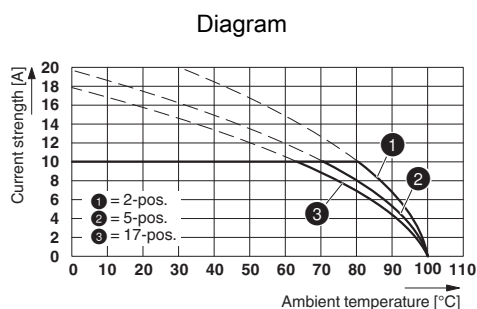
Type: MSTB 2,5/...-STF-5,08 with MDSTB 2,5/...-GF-5,08
