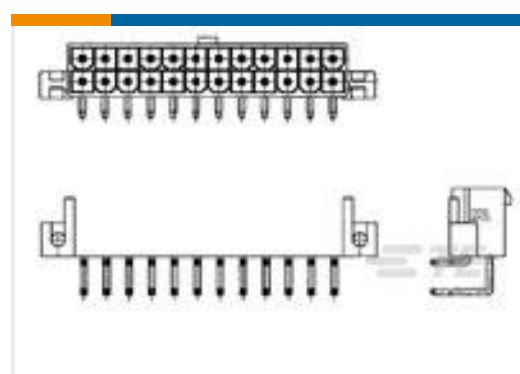
TE Part #1586044-2 2P VAL-U-LOK R/A HDR SCR MT V0
