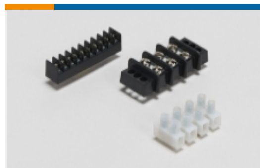
Barrier Strips(272)
