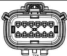
2X6 WITH CLIPSLOT *
