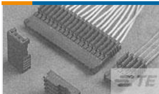
TE Part #281783-5 PLUG HE14 IDC 180 5 P AWG 26-24
