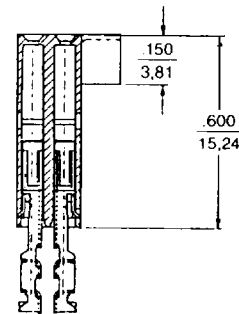
Section C-C
