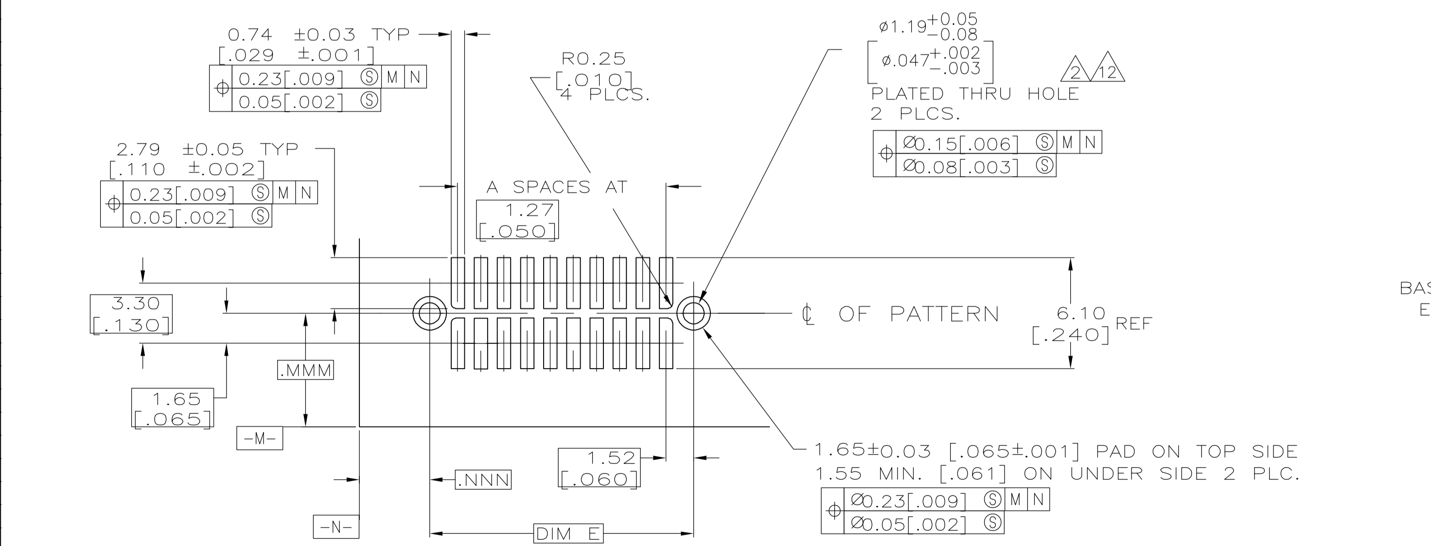
RECOMMENDED BOARD LAYOUT SCALE: 5:1
