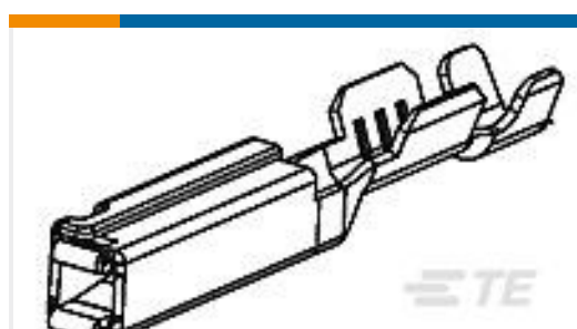
TE Part #1123343-2 TH/.025 CONNECTOR SYSTEM, RECEPT AND TAB
