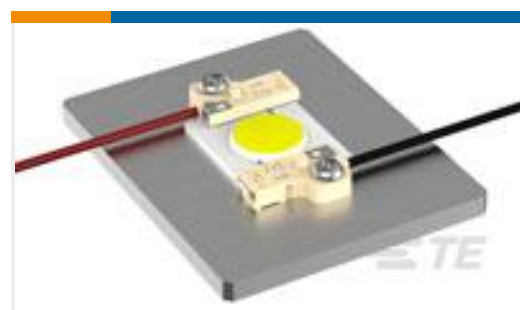
TE Part #2134318-1 LUMAWISE LED HOLDER, TYPE LUMIPACK N1
