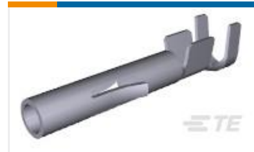
TE Part #350536-2 UMNL SOK 20-14 .0126 AUNI/BR
