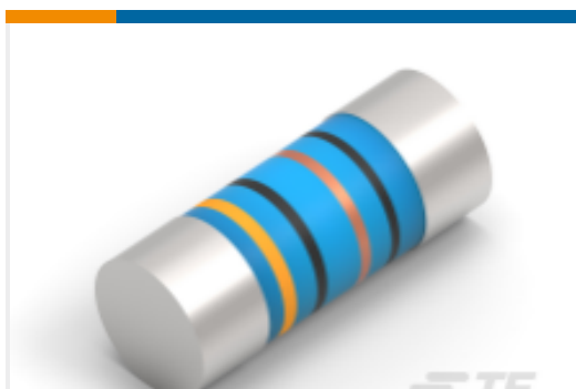
TE Part #9-2176314-0 MELF SMA-A 390K 1% 50PPM 0102 0.3 W
