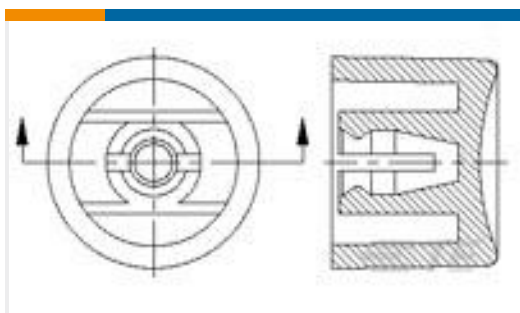
TE Part #4-643813-1 Nylon Tin Plated Receptacle: 2.54mm, With Mating Alignment, MTA 100
