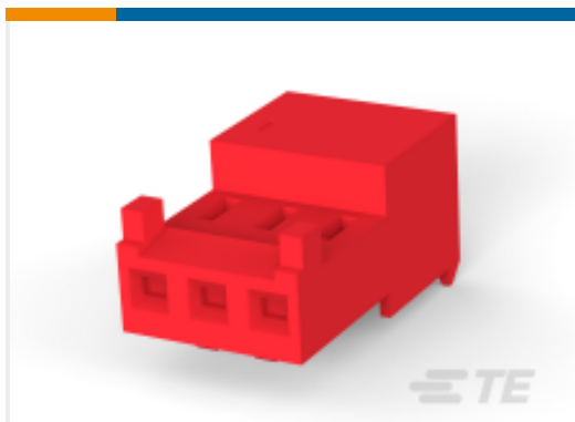
TE Part #4-643813-1 Nylon Tin Plated Receptacle: 2.54mm, With Mating Alignment, MTA 100
