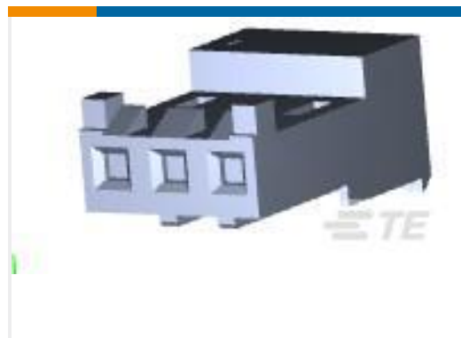
TE Part #3-643817-3 03P MTA156 CONN ASSY 18AWG ORA
