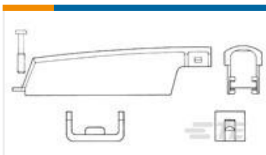
TE Part #4-229910-1 CLAMP, CABLE
