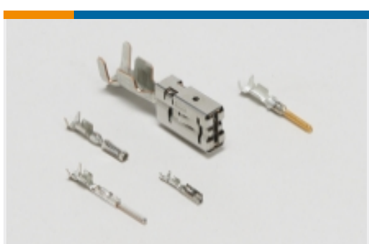
Automotive Terminals(82)
