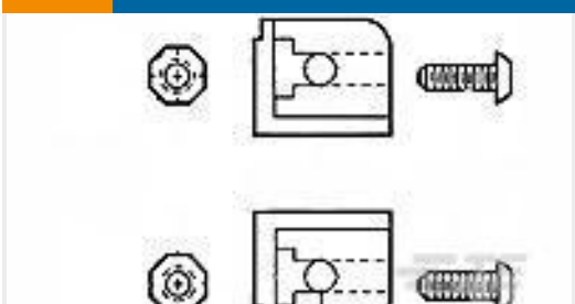
TE Part #533050-1 HDI MOUNTING EAR KIT
