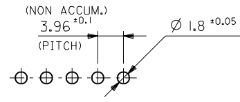
RECOMMENDED P.C.BOARD HOLE DIM.
