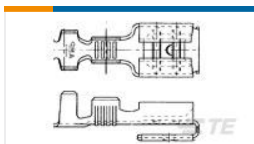
TE Part #280232-8 250 FASTON POST INS.,REC.,1 POS, NATRUAL
