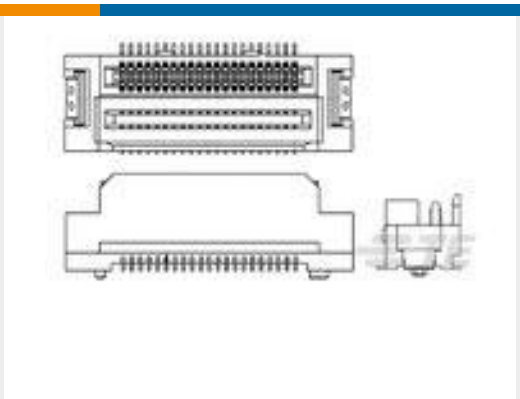
TE Part #2069389-1 Z-STACK CONN. 42P ASS'Y F8
