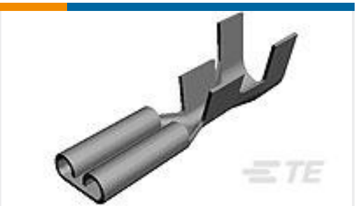
TE Part #42566-1 187 FASTON REC 20-16 AWG BR
