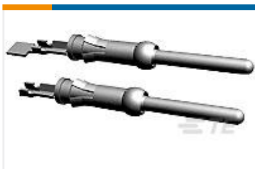
TE Part #1-66099-2 III+ PIN,18-16,TIN-LEAD,SMPACK
