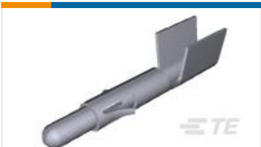
TE Part #350922-3 PIN, MATE-N-LOK, UMNL
