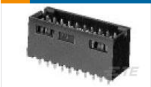
TE Part #2-102618-3 50 MODII HDR DRST SHRD .100CL
