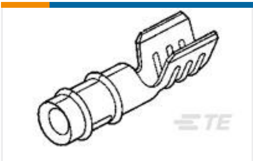
TE Part #640259-1 058 PIN REC IS 18-22 010TPBECU
