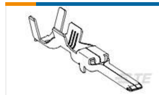
TE Part #1326031-5 2.8MM BLD,SEAL,14AWG
