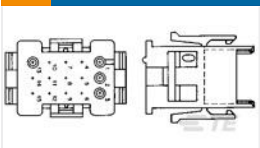
TE Part #1-640511-0 09P MR II CAP HSG V0 RED
