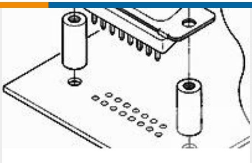
TE Part #5205933-3 BUSHING KIT
