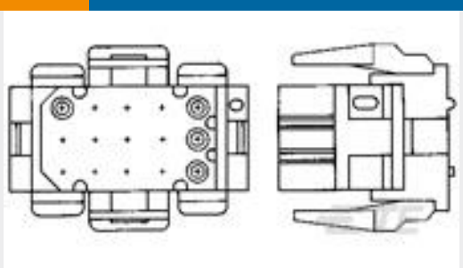
TE Part #1-640522-0 12P MR II PLUG HSG RED
