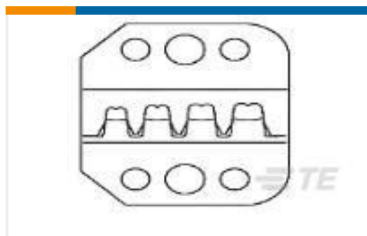
TE Part #90869-2 PROCRMP DIE COMM .062 PIN/SOC
