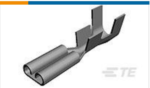
TE Part #41771 250 FASTON REC 22-18 AWG BR
