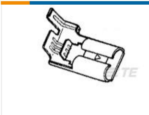
TE Part #1-1627087-0 RECEPTACLE, FLAG QC 4.8x0.8 (H25411)
