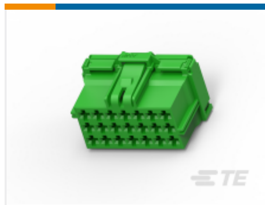
TE Part #4-968975-1 AMP MCP, UNSEALED CONNECTOR HOUSING
