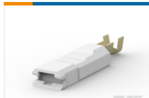
TE Part #1-1969529-1 ULTRA-POD 250 ASSEMBLY REC 18-14 AWG BR
