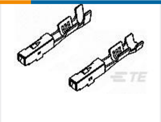
TE Part #1717172-1 040 III RCPT NONSEALED TIN LP
