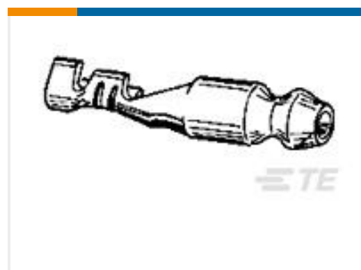
TE Part #153209-2 SHUR PLUG .18 DIA REC 18-16 AWG TPBR
