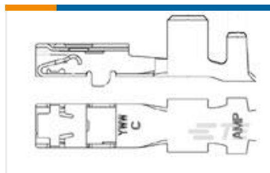
TE Part #1326030-8 2.8MM RECP,UNSEAL,10-12AWG,REV
